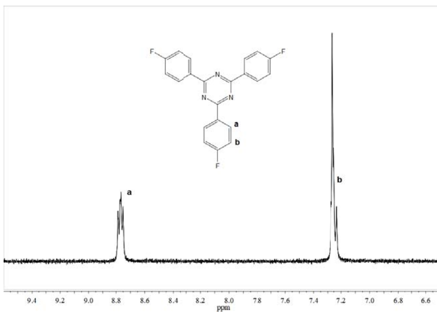
Figure S2. 1 H NMR spectrum for TFPT.
