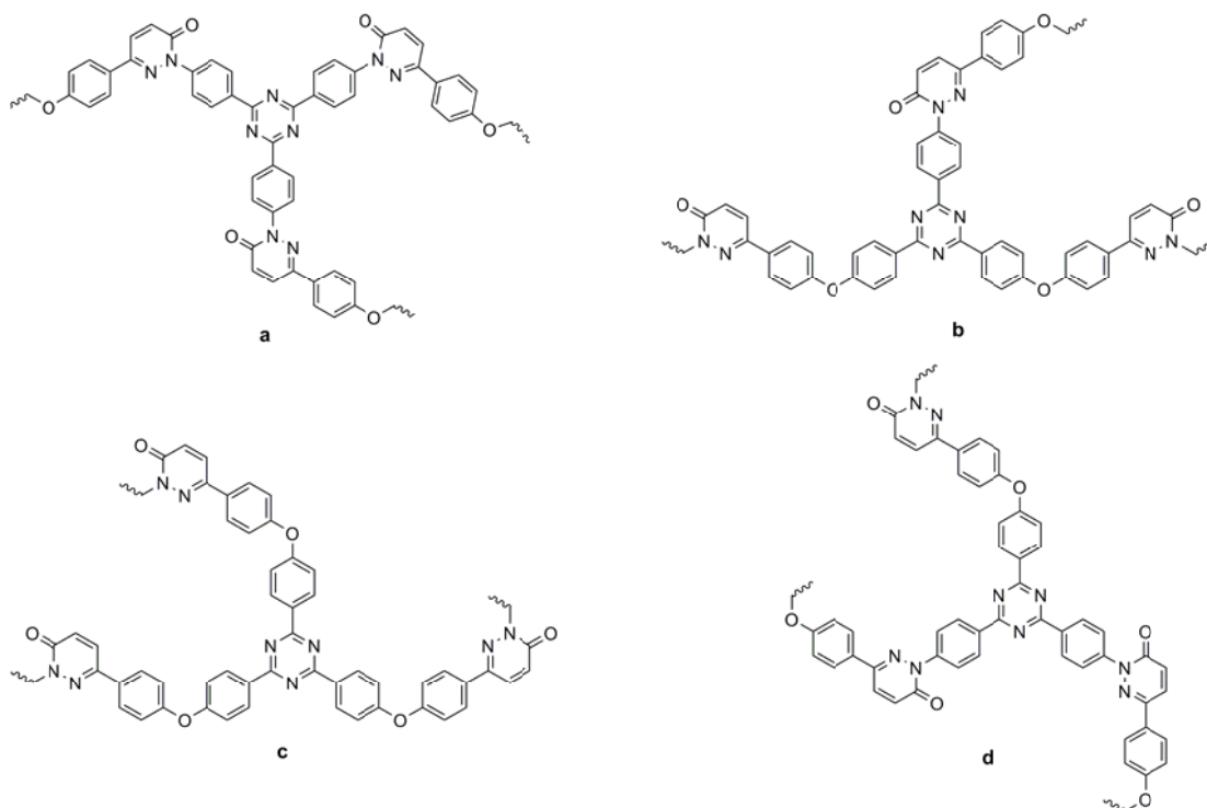
Scheme S1. Chemical formula of the cross-linked polymer.
