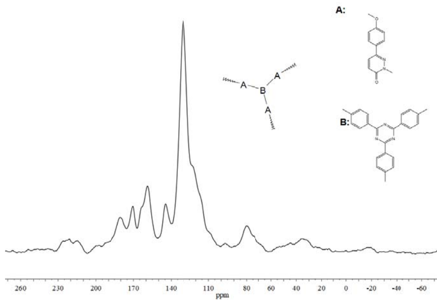
Figure S3. Solid ^{13}\text{C} NMR spectrum for the polymer.
