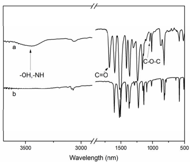
Figure S1. FTIR spectra for polymer (a), and TFPT (b).
