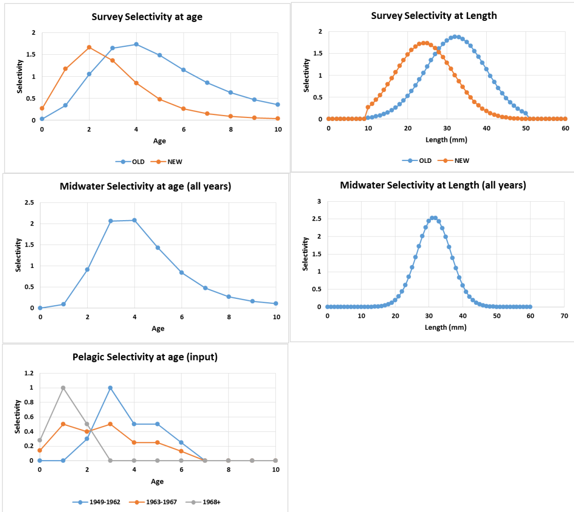
Figure 2: 2019 BC model selectivity functions. The old gear (OLD) survey selectivity plot applies also to the demersal bycatch. Demersal and midwater selectivities are estimated, and the pelagic selectivities input. The values estimated correspond to the 2020 BC assessment.
