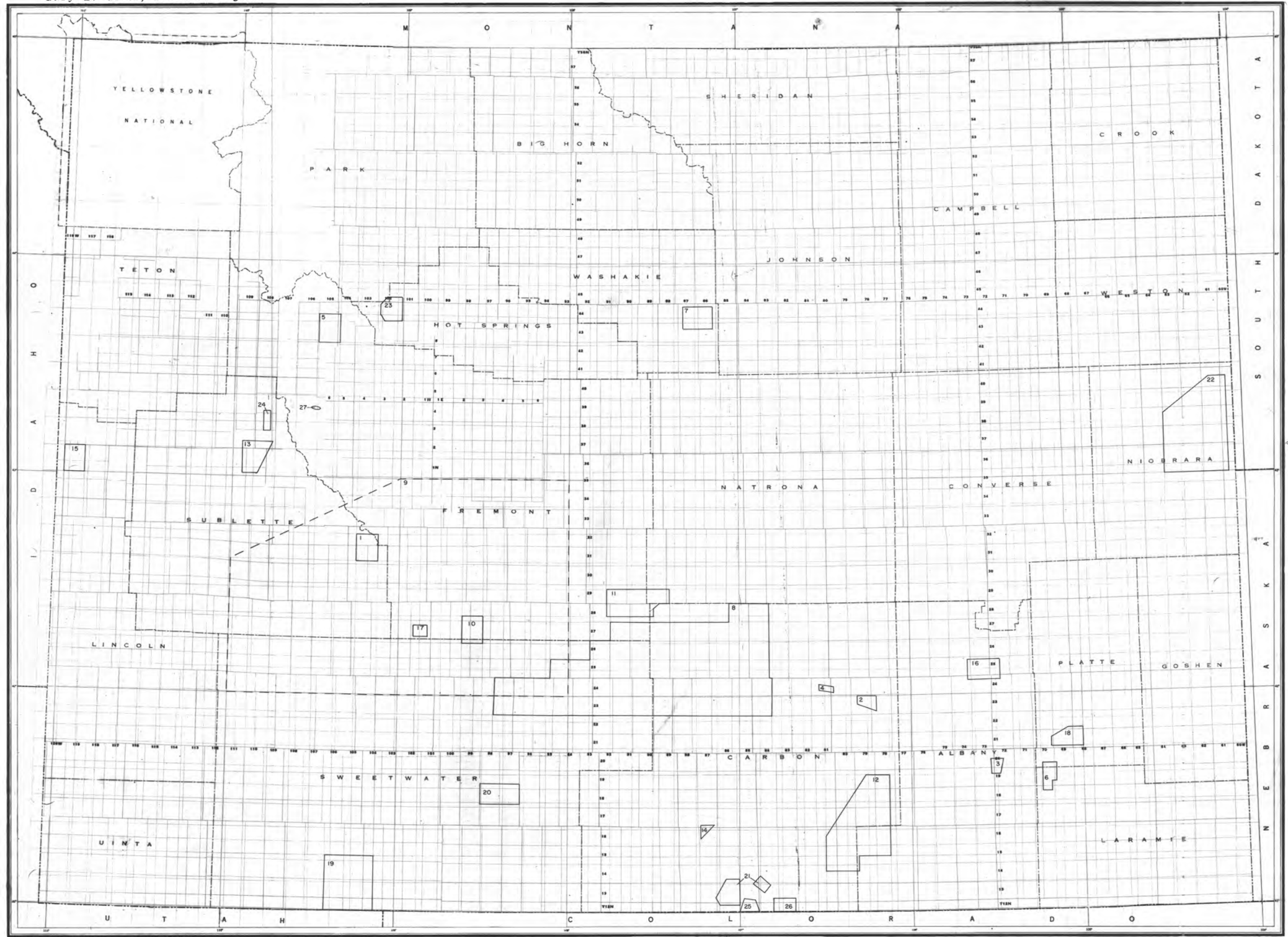
INDEX MAP TO GEOLOGIC MAPS FOR WYOMING INCLUDED IN 1980-1985 GRADUATE THESES FROM THE UNIVERSITY OF WYOMING Compiled by Alan J. Verploeg and Phillip L. Greer, 1986
