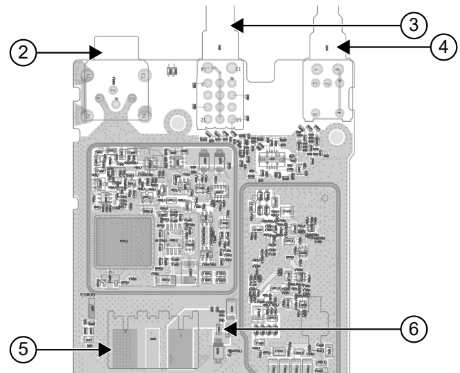
PCB Bottom View
