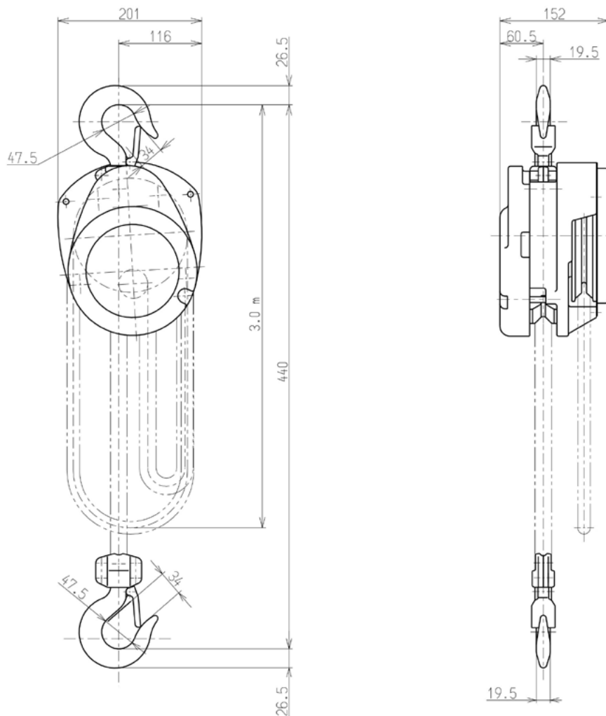
All measurements are in mm
