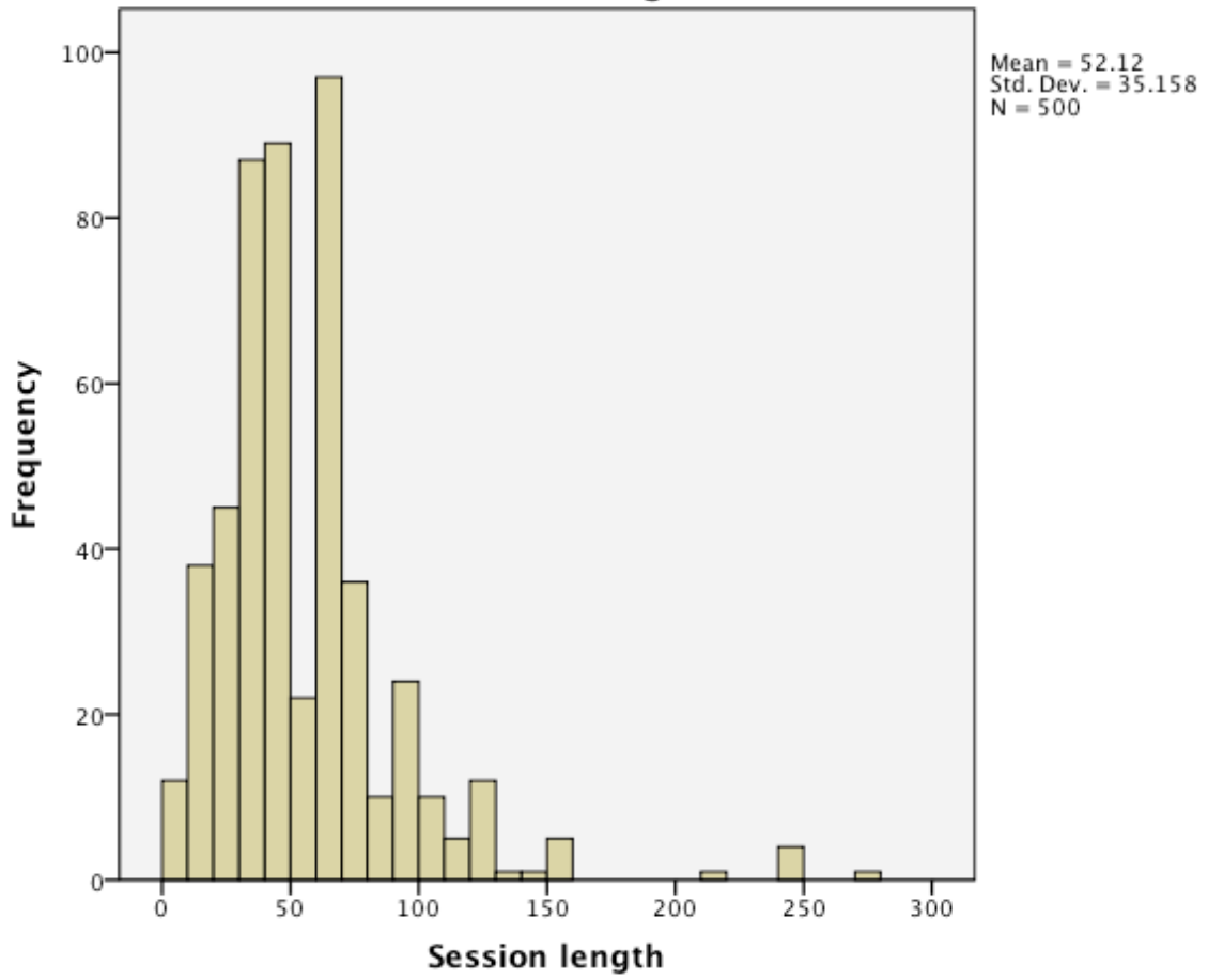
Histogram
