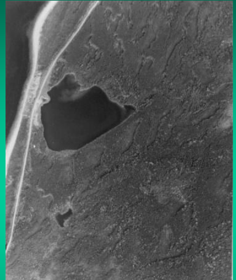
Surface gravity waves (Görtler Vortices ?) inferred from the pattern of a Balsam Fir Wave Forest and windrowing of foam streets on a pond at Spirit Cove, Newfoundland. © Alexander Robertson 1985
