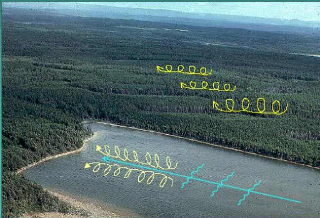
Surface gravity waves (Görtler Vortices ?) inferred from the pattern of a Balsam Fir Wave Forest and windrowing of foam streets on a pond at Spirit Cove, Newfoundland. © Alexander Robertson 1985
