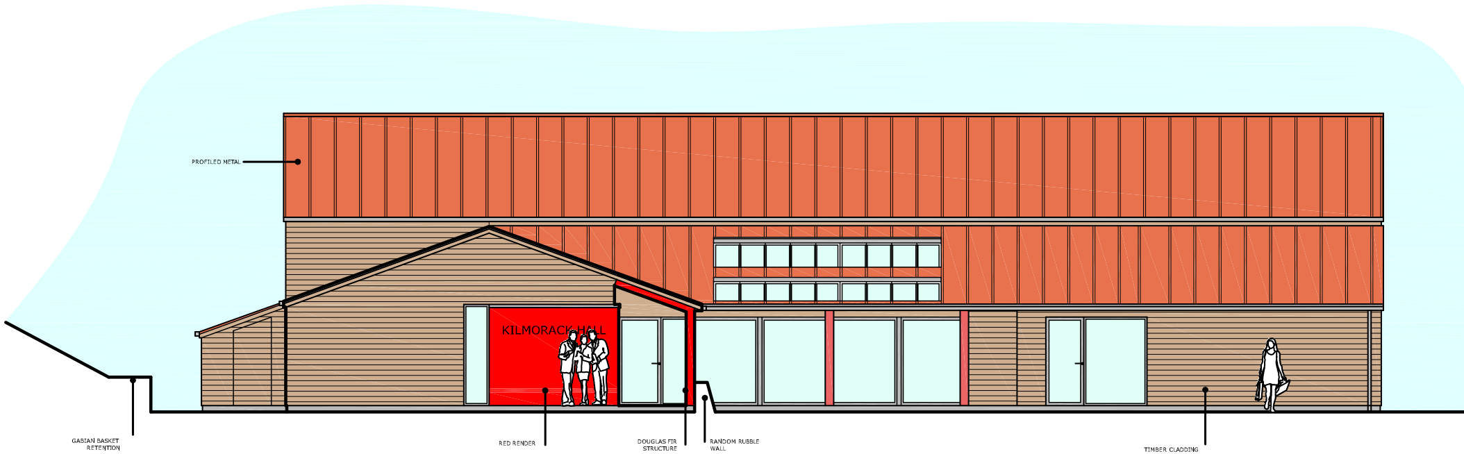
NORTH WEST ELEVATION 1:100
