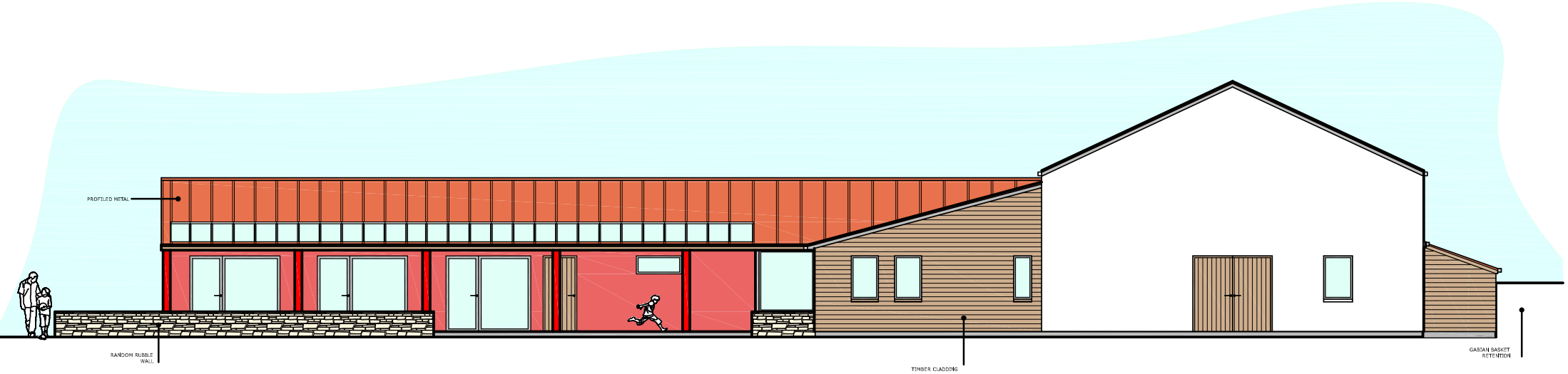
SOUTH WEST ELEVATION 1:100
