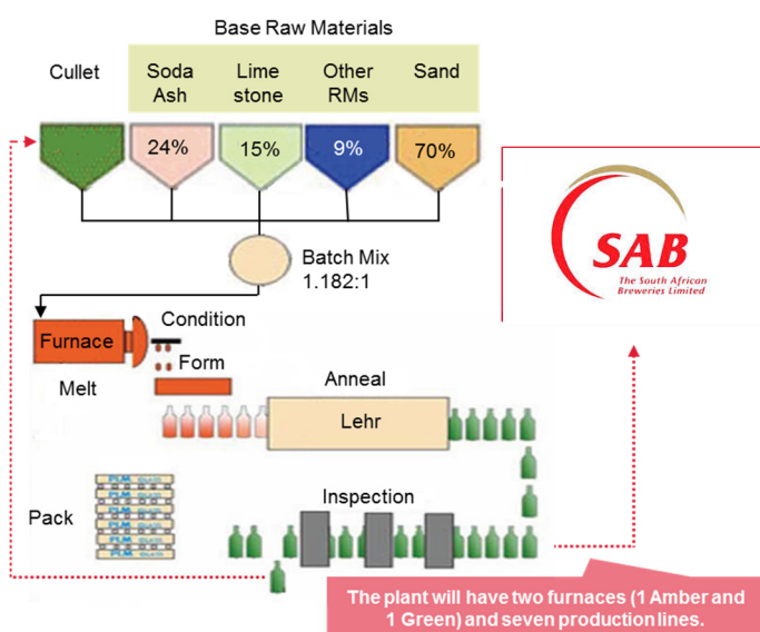
Figure 1-1: Conceptual Process
