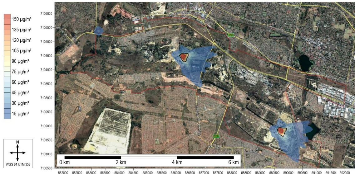
Figure 5-7: Simulated incremental highest daily PM 10 concentrations due to West Wits underground operations
