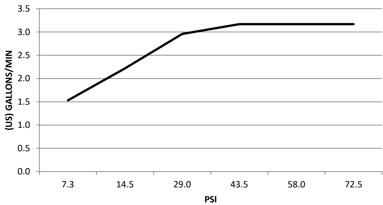
V163 FLOW RATE (US) GALLONS/PSI
