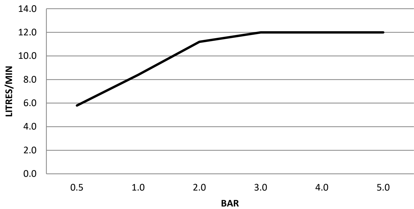
V163 FLOW RATE LITRES/MIN
