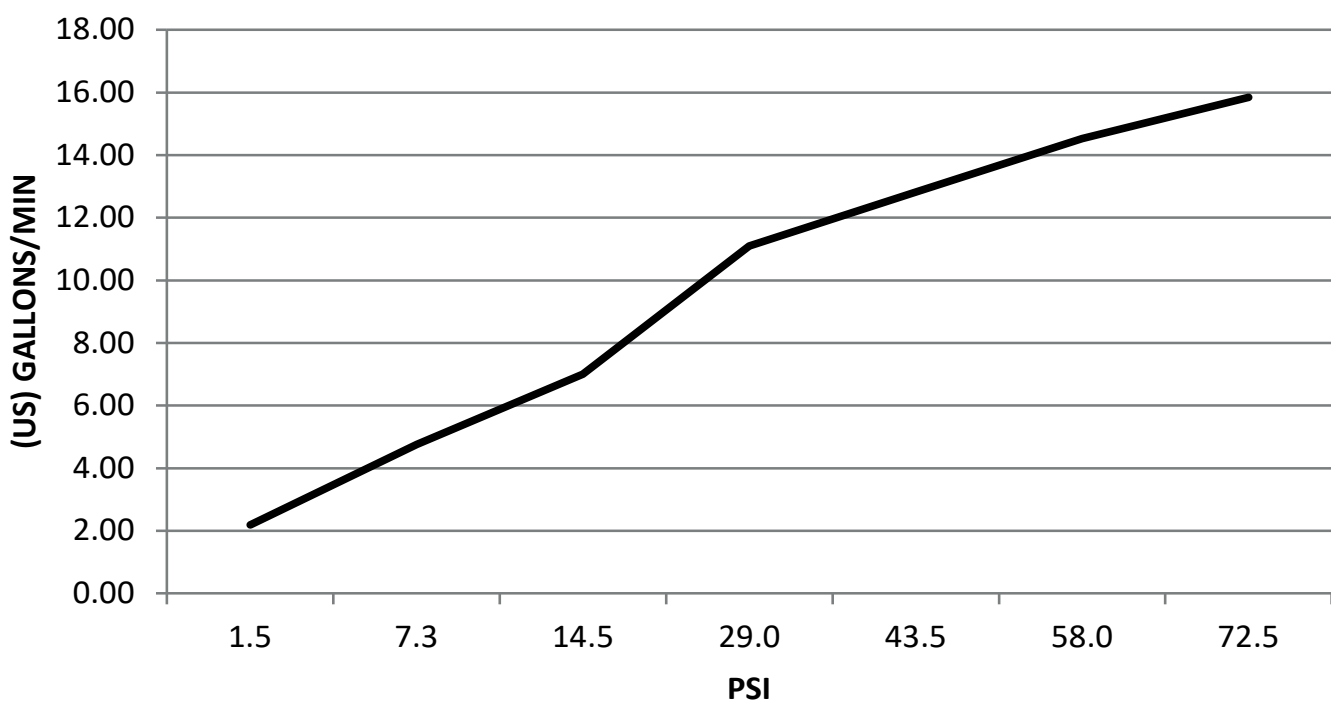
T2046 FLOW RATE (US) GALLONS / PSI
