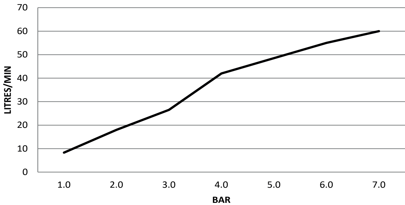
T2046 FLOW RATE LITRES / MIN
