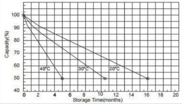
Self-discharge Characteristics
