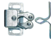
HA70201 Twin Roller Catch, Spring Loaded, Screw Fix
