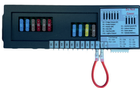
BC18001 2018 Converter Relay Housing with Link Harness
