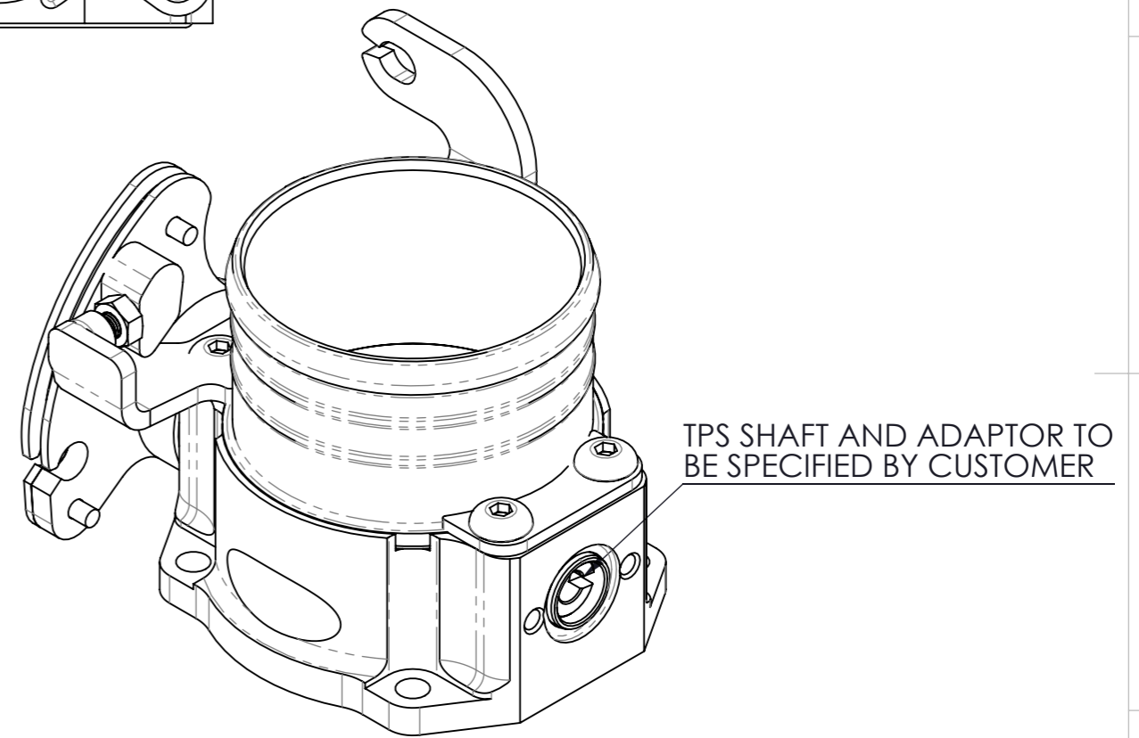
ISOMETRIC VIEW
