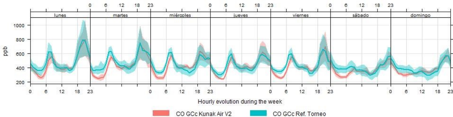
Time variation of Kunak Air V2 and Ref. Torneo : CO GCc
