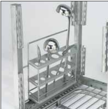
Utensil holder. Part. no. 209.7353 For utensils max 650 mm high.
