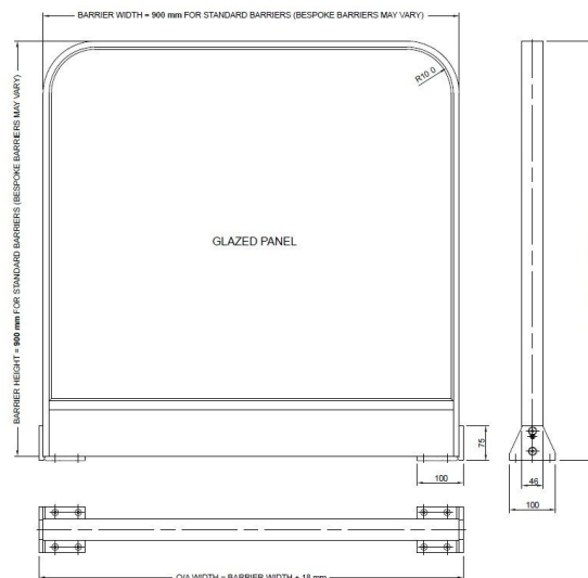
Dimensions drawing (DIM)
