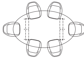
110 cm | 43 1/4" Frame position B
