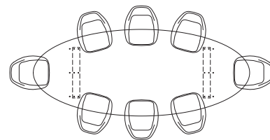
181 cm | 71 1/4" Frame position B
