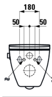
Connection with commercially available installation systems
