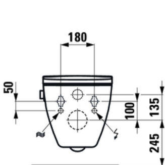
Connection with Laufen installation system LIS CW2
