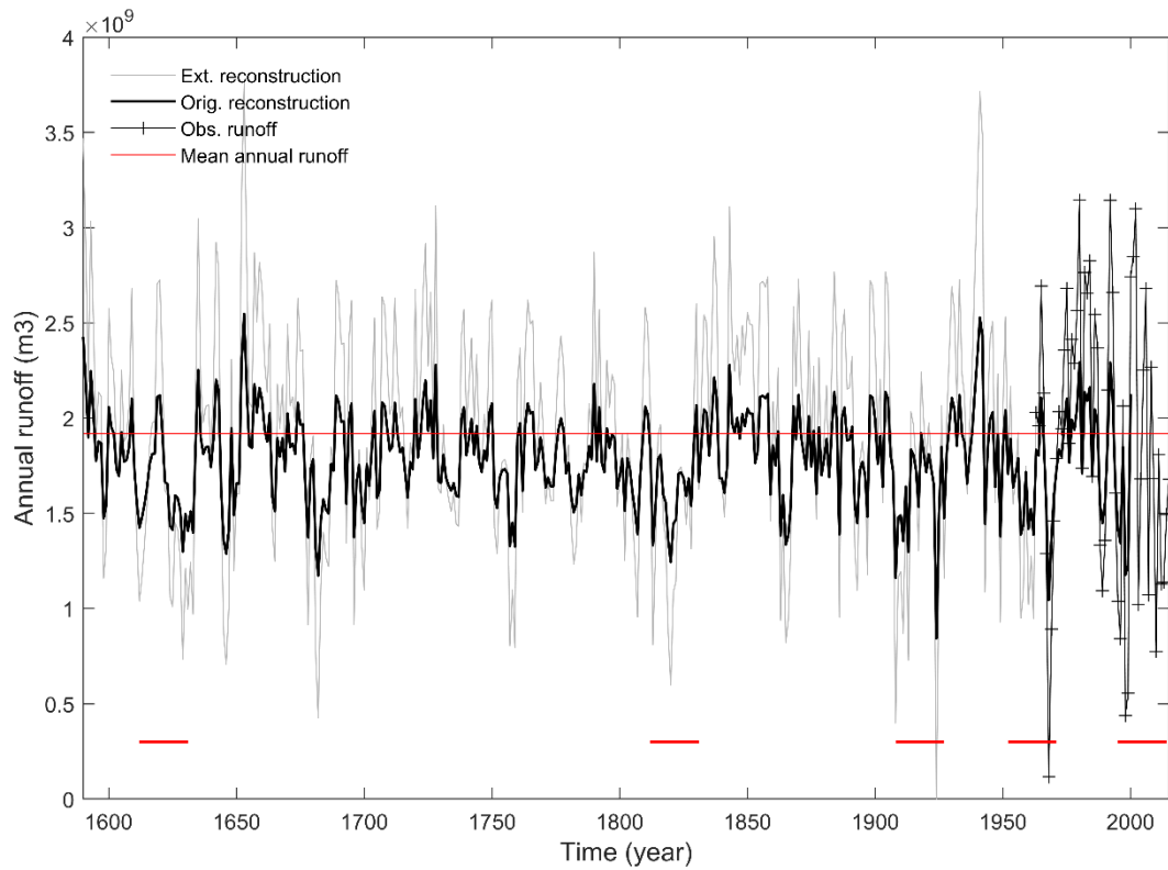
Figure S1. Comparison of original, extended and variance-corrected Perquilauquén at Quella runoff reconstruction. Black line represents the original time series reconstruction for the period 1590-2000. The grey line represents the extended and variance-corrected reconstruction for the period 1590-2015. The horizontal red line indicates mean annual runoff, and red bars indicate the five driest periods identified over the period of reconstruction. Lines with crosses indicate observed or gauged annual runoff at Perquilauquén at Quella.
