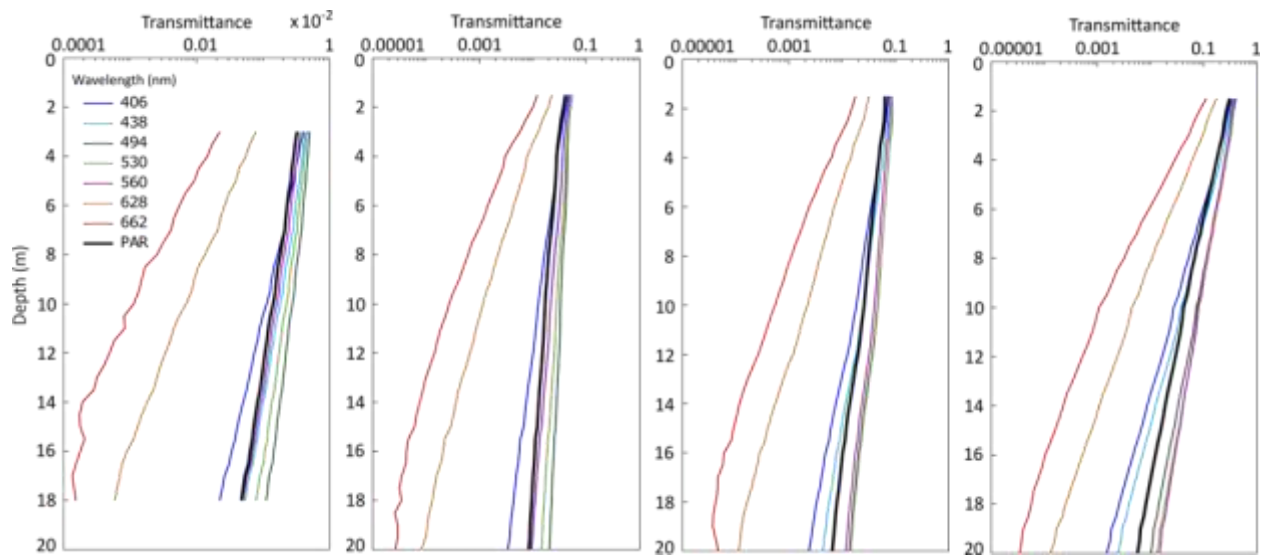
Figure S1. Planar transmittance (PAR) profiles at selected wavelengths. Profiles were measured in the water column beneath landfast sea ice with (a) thick snow cover ( h_S = 29 cm) on 16 May 2015, (b) a thin wet snow cover ( h_S = 11 cm) on 16 June 2016, (c) bare surface on 27 June 2016 and (d) ponded surface ( h_{MP} = 4 cm) on 4 July 2016. Note the different transmittance scales.
