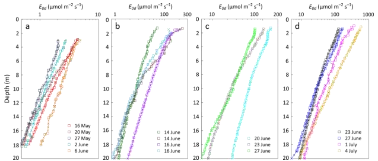
Figure S2. Vertical profiles of downwelling PAR. Interpolated (x) and measured (square) downwelling scalar PAR beneath (a) snow-covered sea ice in 2015, and (b) snow-covered ice, (c) white ice and (d) ponded ice in 2016.
