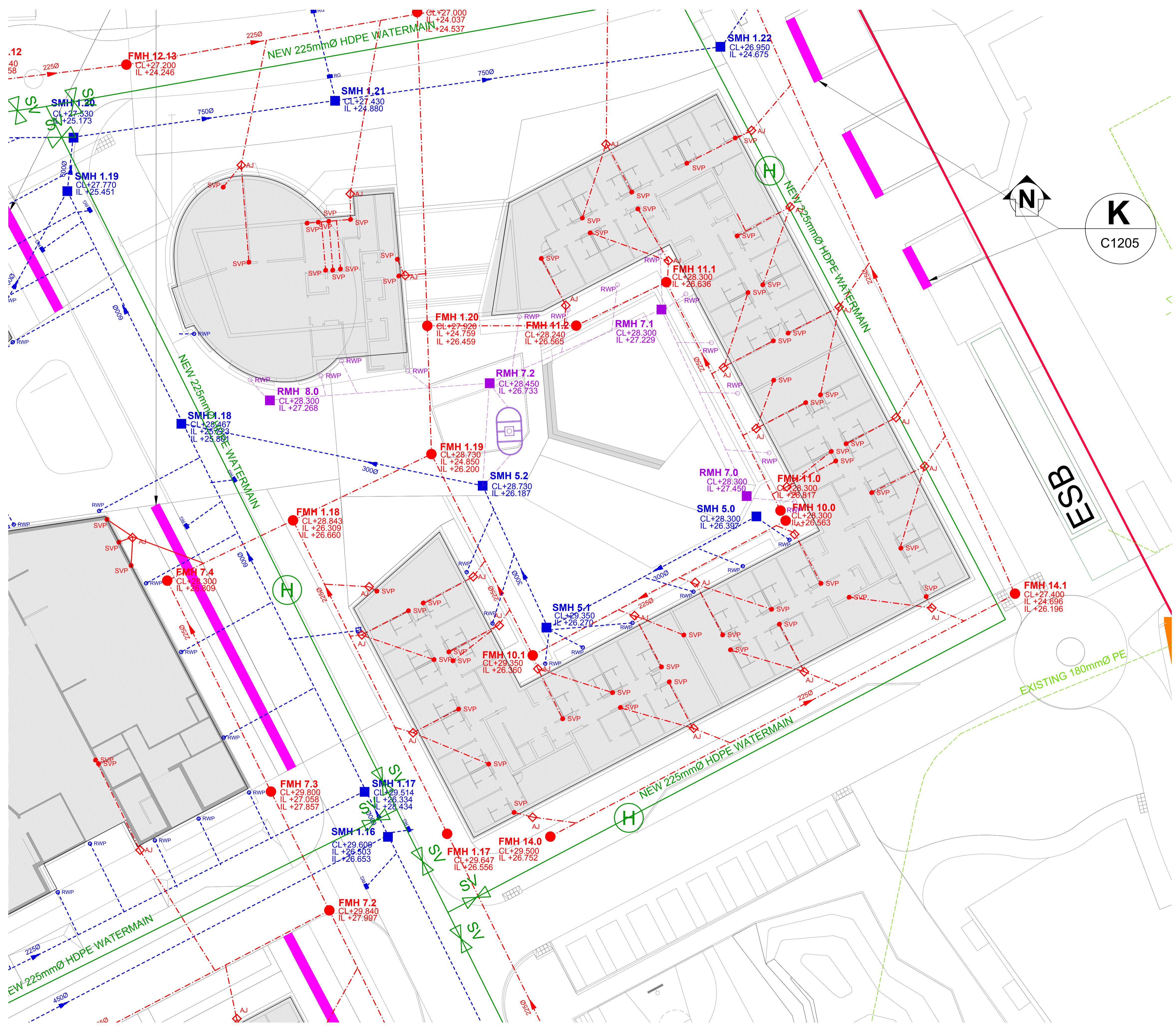
PROPOSED DRAINAGE AND WATERMAIN LAYOUT SCALE @ A1: 1:200 SCALE @ A3: 1:400
