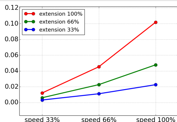
Stopafstand i meter for 66% for 16 kg
