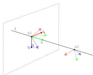
CF :24.3: Definition of the line feature
