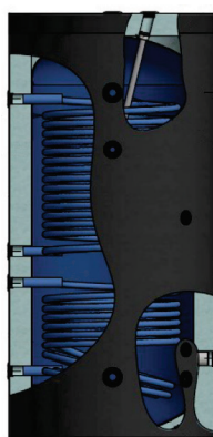
REMOVABLE INSULATION DETAIL ON 800÷1000
