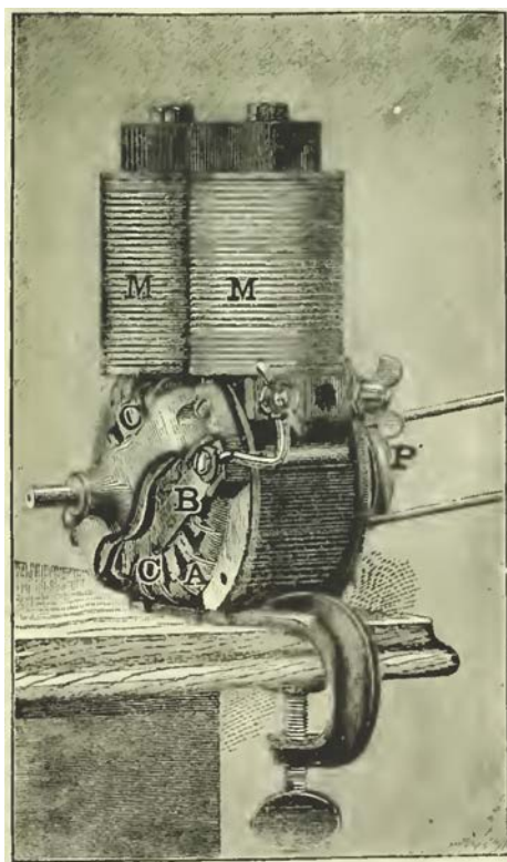
Fro. 109-ELECTROSTATIC [oToR.
