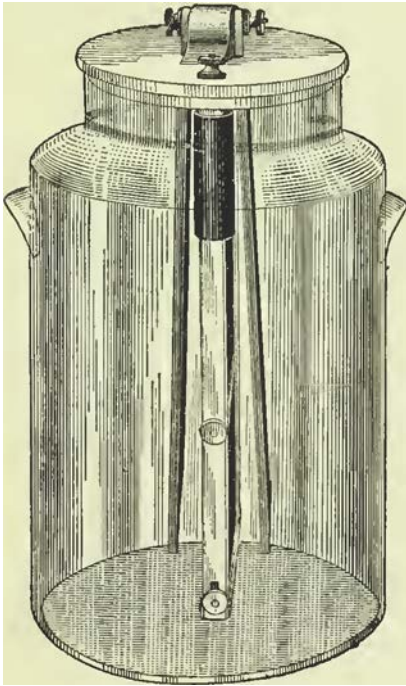
Fm. 14. Emson-LALANDE CAUTERY CELL.
