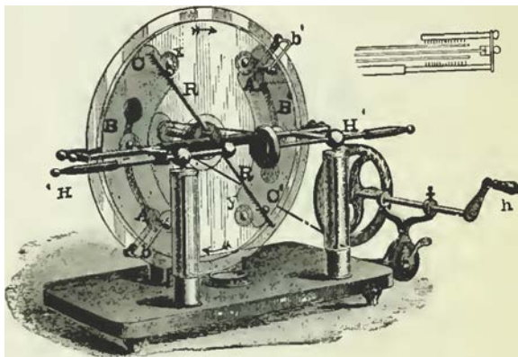
FIG. 69.—SINGLE-PLATE TOEPLER-HOLTZ ELECTRICAL MACHINE.
