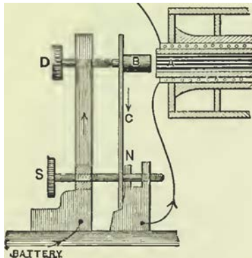
FIG 100.-ADJUSTABLE VIBRATOR FOR FARADIC COILS.
