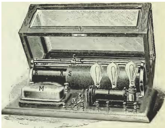
FIG. 114.-ADAPTER FOR CONTINUOUS CURRENT CIRCUITS.
