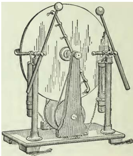
FIG. 72.-BOXE'S ELECTROSTATIC INFLUENCE MACHINE.
