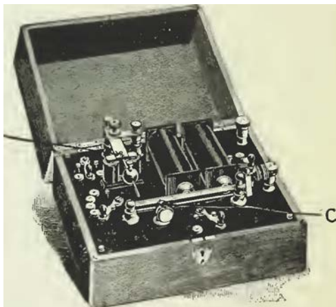
FIG. 101.—INDUCTION COIL WITH RIBBON VIBRATOR.
