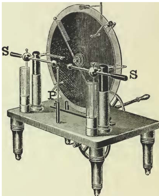
Fro. 146.-ELECTROSTATIC INFLUENCE MACHINE FOR EXCITING X-RAY TUBES.
