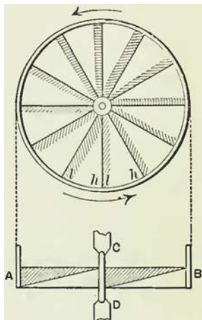
Fig. 83.-MECHANICAL MODEL HAVING ANALOGIES WITH ELECTRIC CIRCUIT.
