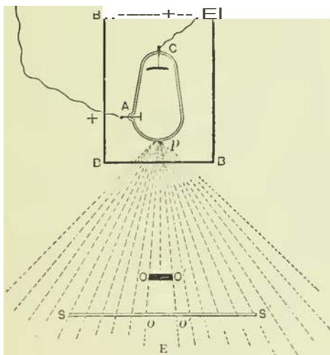
FIG. 130.—ILLUSTRATING USE OF FLUORESCENT SCREEN.
