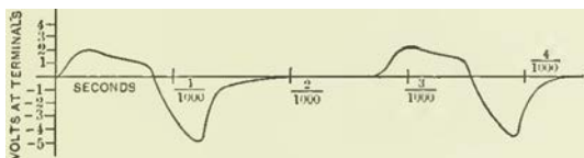
FIG. 97.—TYPE OF SECONDARY INDUCED E.M.F. AT LOW FREQUENCY. (See also Fig. 90.)
