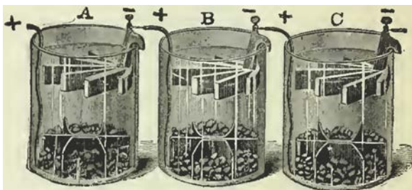
FIG. 17.-SERIES CONNECTION OF THREE DANIELL GHAYITY CELLS.
