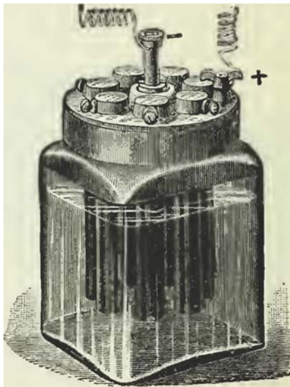
FIG. 11.—ZINC-CARBON CELL.
