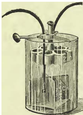
FIG. 7.—BLUESTONE OR GRAVITY VOLTALIC CELL.
