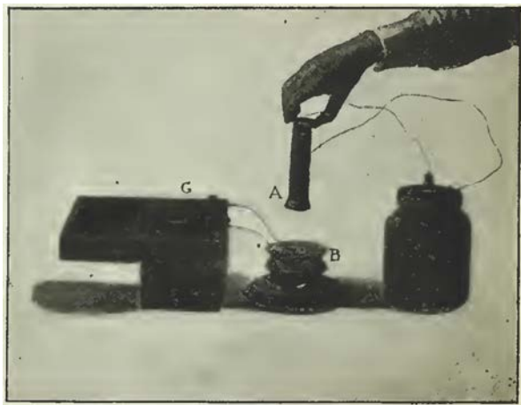
FIG. 85.-MUTUAL INDUCTION.
