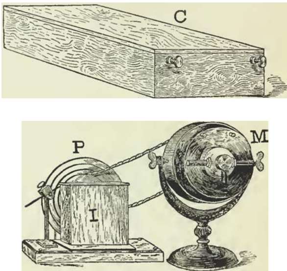
FIG. 138.—CORNENSETT AND HOLTZ'S CONDENSER.
