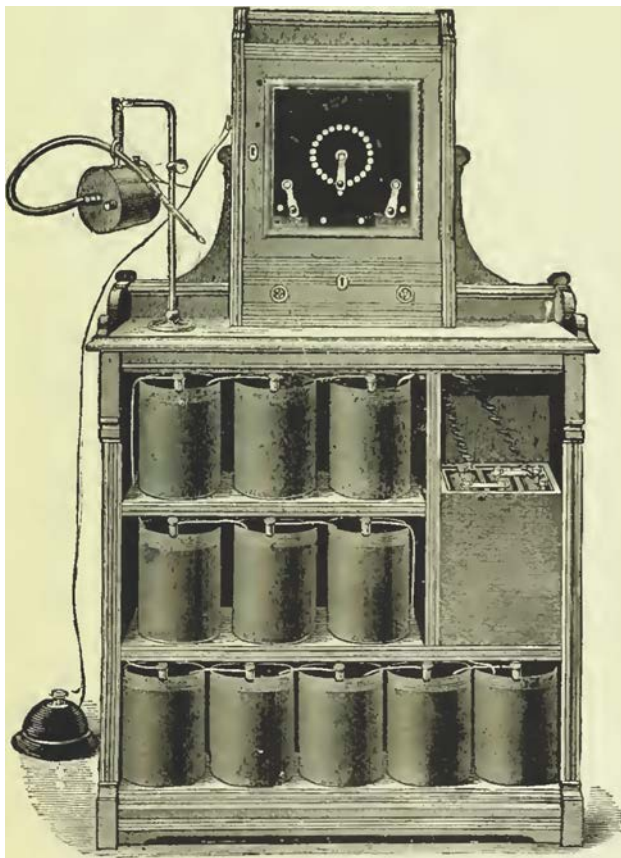
FIG. 25 - C. W. NET CONTAINING ELEVEN PRIMARY VOL- TAGE CELLS FOR CHARGE OF TWO STORAGE CELLS.
