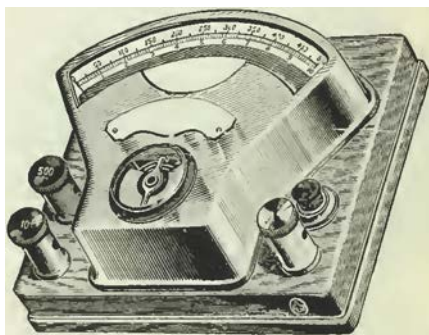
FIG. 33.-"WESTON MAGNETOMETER.
