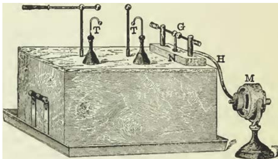
FIG. 144.-X-RAY TRANSFORMER FOR ALTERNATING CURRENT CIRCUIT.
