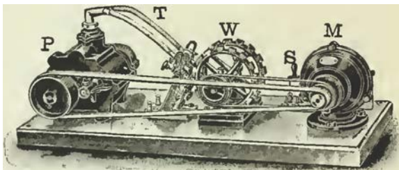
Fig. 139.-INSTANTANEOUS AIR-BREAK WHEEL.
