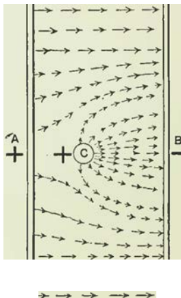
FIG. 59.-DIAGRAMMATIC REPRESENTATION OF ELECTRO-STATIC FLUX PATHS.
