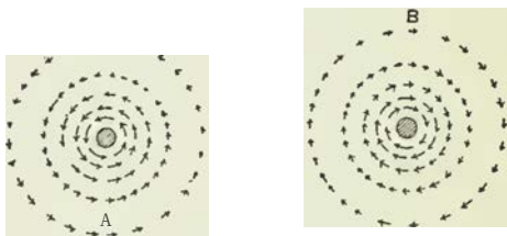
Fra. 75.-MAGNETIC FLUX PATHS SURROUNDING A STRAIGHT ACTIVE CONDUCTOR.
