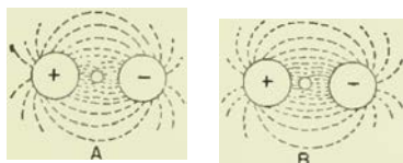
FIG. 61.-EFFE<'T OF UNCLHIGED SPHERE.
