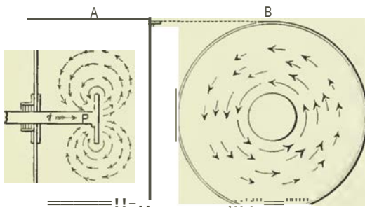
FIG. 7.-HYDRAULIC ANALOGY OF THE RELATION BETWEEN ELECTRICITY AND MAGNETISM.
