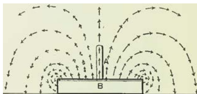
FIG. 64.-REPRESENTING ACTION AND OPERATION OF ELECTROPHORUS.
