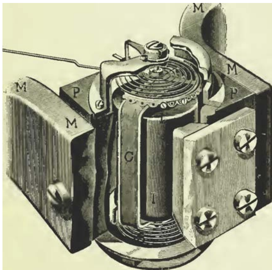
FW. 34.--WORKING PARTS OF WESTINGHOUSE DYNAMOMETER.
