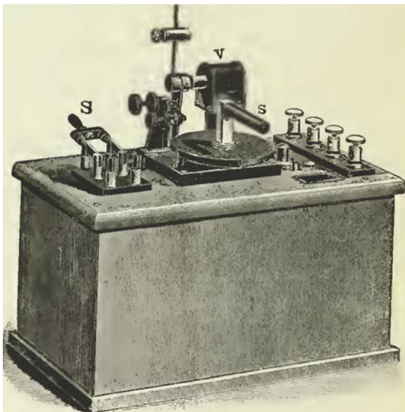
FIG. 142. VARIATOR AND CURRENT-CONTROLLING SWITCHES.
