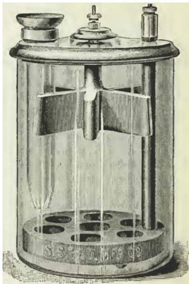
FIG. 15.-PAUTZ GRAVITY CELL.
