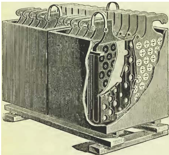
FIG. 22.—INTERNAL VIEW OF CHARGING STORAGE BATTERY.
