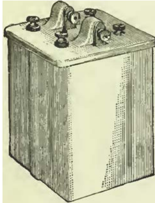
FIG. 18.-EDISON-LALANDE BATTERY.
