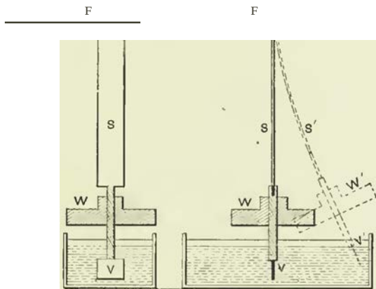
FIG. 124.-MECHANICAL VISCOSITY, SIDE AND END VIEW.
