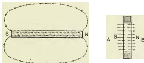
FIG. 76.—DIAGRAM OF FLUX PRODUCED BY PERMANENT MAGNET AND BY CURRENT OF ACTIVE COIL.
