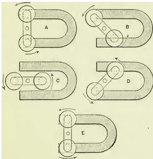
FIG. 89.—DIAGRAMS REPRESENTING CHANGES IN THE MAGNETIC CIRCUIT OF MAGNETO-ELECTRIC GENERATOR.
