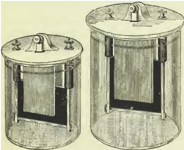
Fig. 13.-Emson-LALANDE CELLS.
