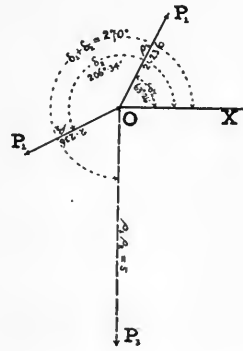
FIG. 10. — Product of two Complex Quantities, Polar Coördinates 2.236 / 63^\circ.26' \times 2.236 / 206^\circ.34' = 5 / 270^\circ = OP_3
