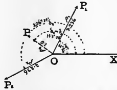
FIG. 11. — Quotient of two Complex Quantities, Polar Coördinates.
