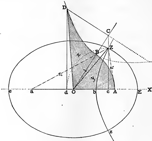
FIG. 22. — Constructions for \cosh (x \pm iy) and \cosh^{-1}(u \pm iv) .
