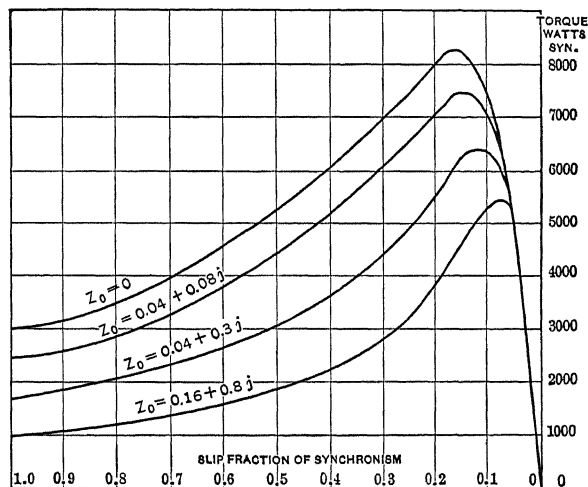
FIG. 46.—Induction-motor speed torque characteristics with short-circuited secondary.
