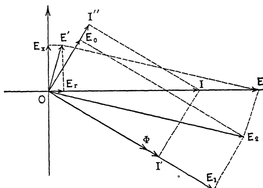
FIG. 178.—Single-phase commutator motor. Unity power-factor produced by lagging e.m.f. of rotation.
