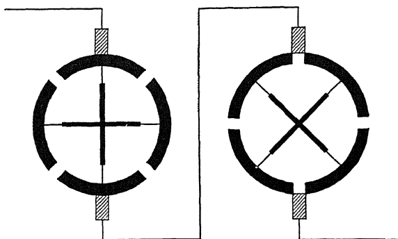
FIG. 119.—Rectifying commutators of the Brush arc machine.
