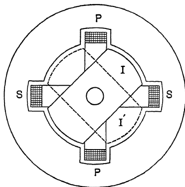
FIG. 145.—Magneto commutation voltage regulator.
