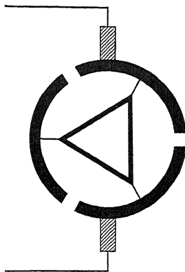
FIG. 107.—Three-phase delta-connected rectifier.
