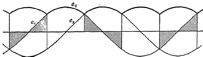
Fig. 112.—Voltage waves of quarter-phase star-connected rectifier.
