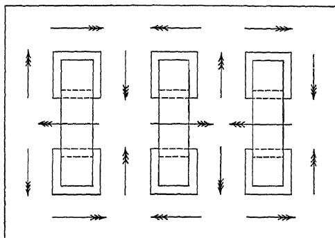
FIG. 207.—Shell-type transformers.
