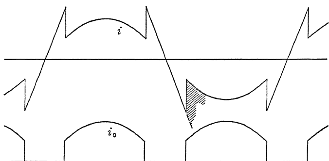
FIG. 86.—Current waves of short-circuit rectifier on non-inductive load.
