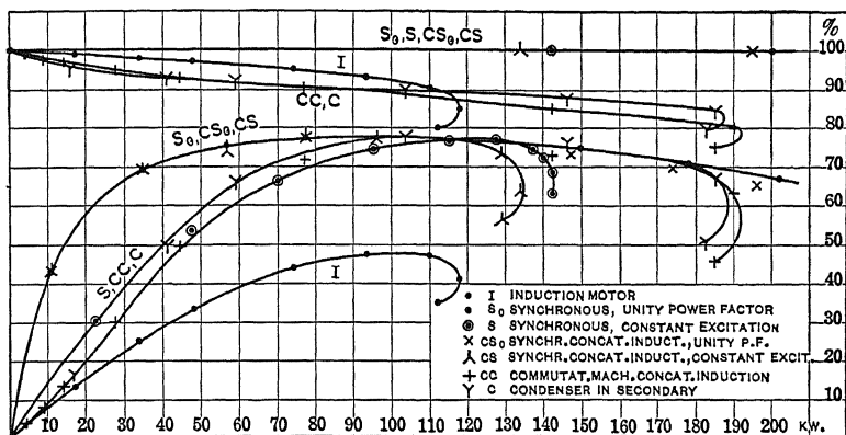
FIG. 28.—Comparison of apparent efficiency and speed curves of high-excitation induction motor with various forms of secondary excitation.
