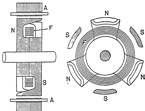
FIG. 146.—Semi-inductor type of machine.
