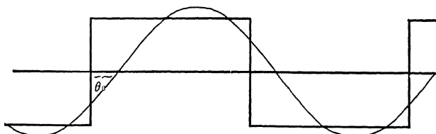
FIG. 213.—Alternating and direct current in a coil midway between adjacent collector leads.
