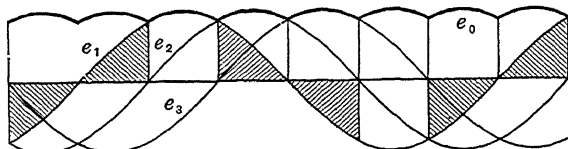
FIG. 117.—Voltage waves of six-phase star-connected rectifier.
