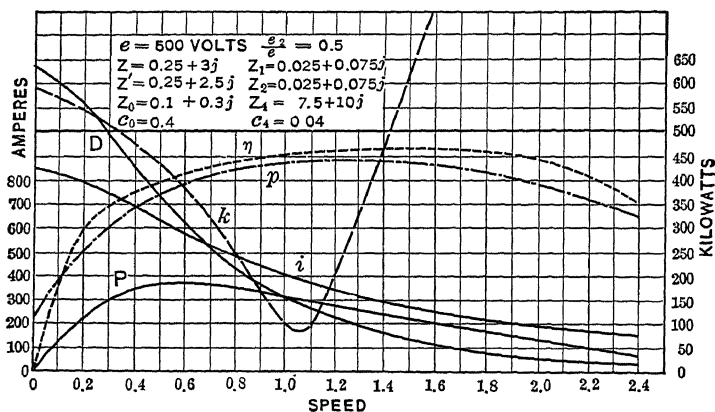
FIG. 191.—Series repulsion motor.
