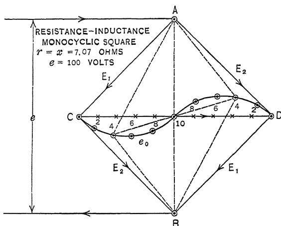
FIG. 67.—Resistance-inductance monocyclic square, topographical regulation characteristic.
