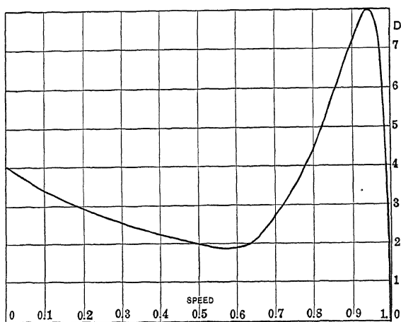
FIG. 53.—Speed-torque characteristic of single-phase induction motor.
