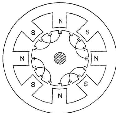
FIG. 134.—Revolving armature alternator
