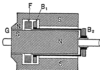
FIG. 222.—Drum type of unipolar machine with revolving magnet core and auxiliary cylinder gap, section.
