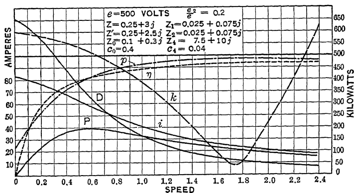
FIG. 190.—Series repulsion motor.
