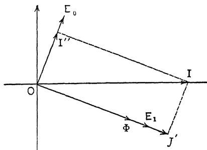
FIG. 177.—Single-phase commutator-motor improvement of power-factor by introduction of lagging e.m.f. of rotation.
