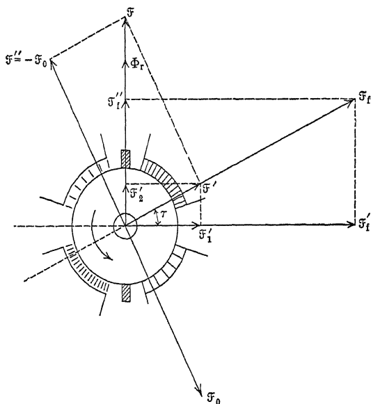
FIG. 202.—Diagram of m.m.fs. in split-pole converter.
