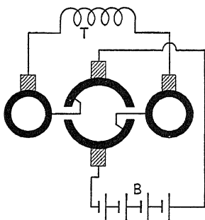
FIG. 95.—Reversing rectifier with alternating-current rotor.
