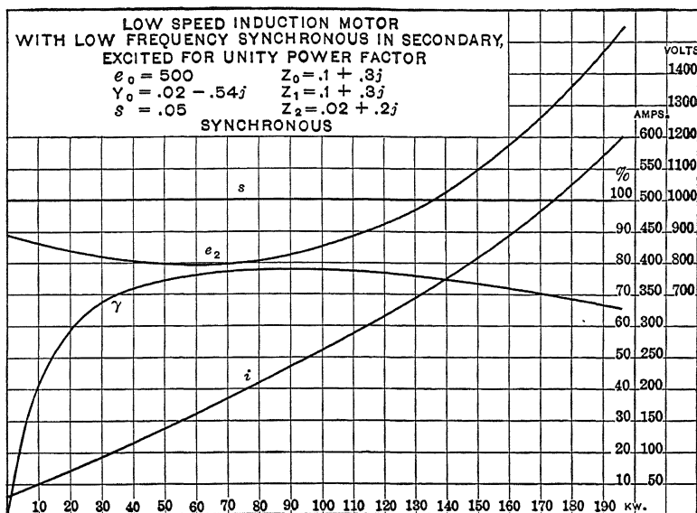
FIG. 29.—Load curves of high-excitation induction motor concatenated with synchronous, at unity power-factor excitation.
