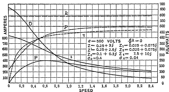
FIG. 189.—Inductively compensated series motor.
