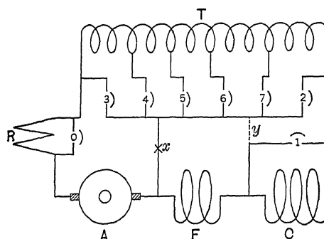
FIG. 182.—Alternating-current commutator motor arranged to operate either as series or repulsion motor.
