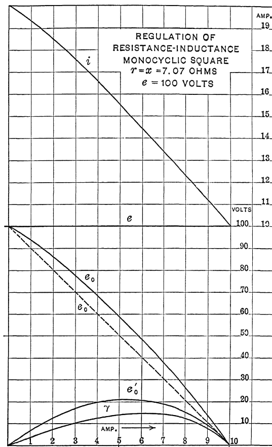
FIG. 68.—Resistance-inductance monocyclic square, regulation curve.
