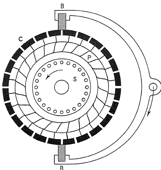
FIG. 60.—Diagram of rotary terminal single-phase induction motor.
