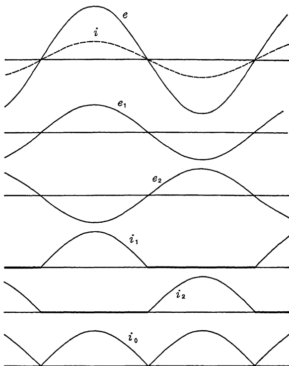
FIG. 100.—Voltage and current waves of contact-making rectifier with direct-current rotor.
