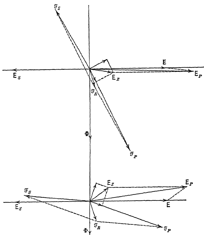
FIG. 166.—Transformer diagram, inductive and non-inductive load.
