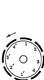
FIG. 224.—Multi-conductor unipolar machine, cross-section.
