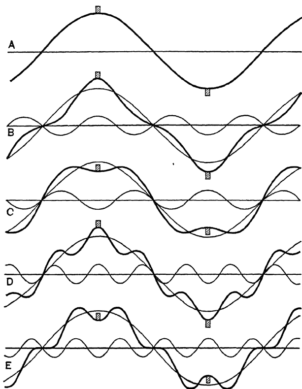
FIG. 205.—Superposition of harmonics to change the e.m.f. ratio.
