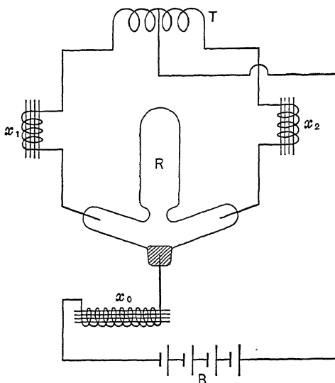
FIG. 102.—Diagram of mercury-arc rectifier with its reactances.
