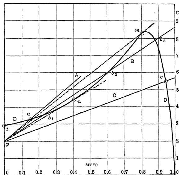
FIG. 52.—Speed torque characteristics of induction motor and load for determination of the stability point.
