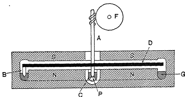
FIG. 227.—Unipolar motor meter.
