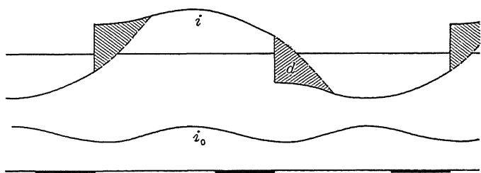
FIG. 89.—Current waves of short-circuit rectifier on highly inductive load, showing sparking but no flashing.
