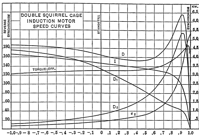
FIG. 14.—Speed curves of double squirrel-cage induction motor.
