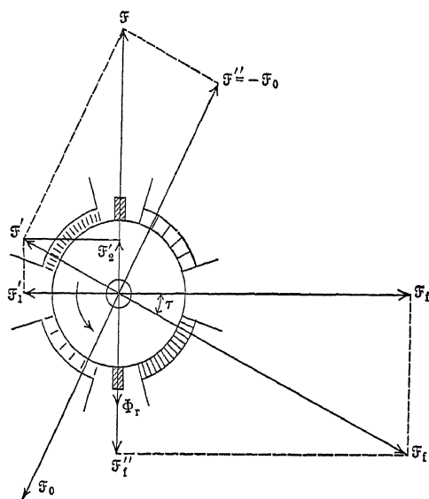
FIG. 203.—Diagram of m.m.fs. in split-pole converter.
