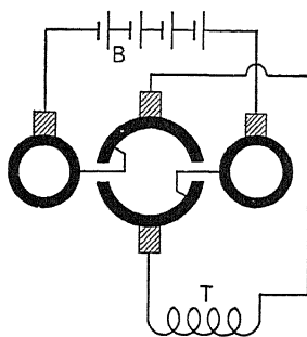
FIG. 96.—Reversing rectifier with direct-current rotor.
