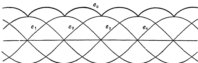
FIG. 113.—Voltage waves of water-phase ring-connected rectifier.
