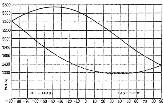
FIG. 66.—Synchronous induction generator, voltage regulation with power-factor of load.
