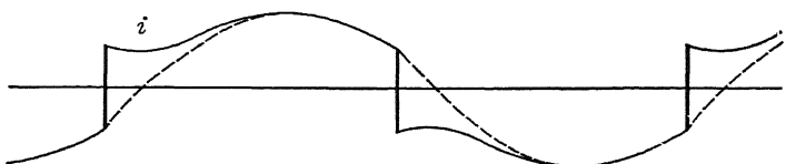
FIG. 76.—Alternating supply wave to rectifier on inductive load.
