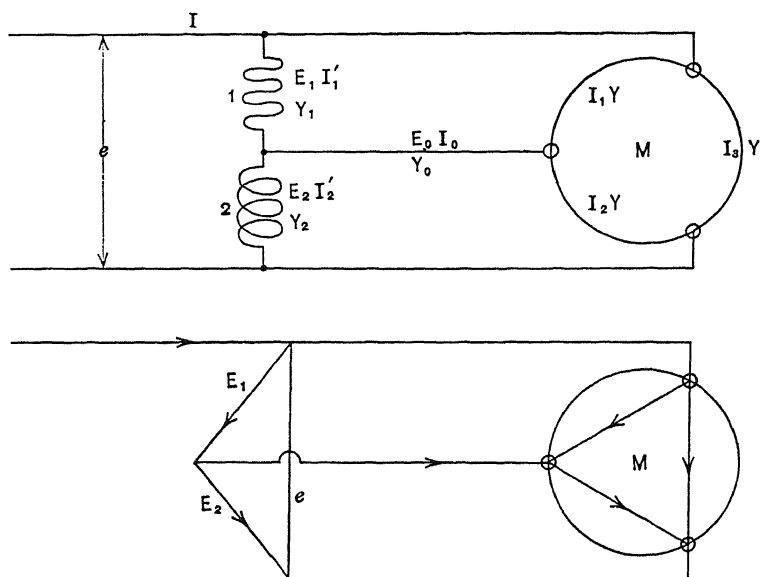
FIG. 42.—Three-phase motor with monocyclic starting device.
