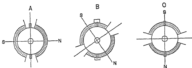
FIG. 198.—E.m.f. variation by mechanically shifting the poles.
