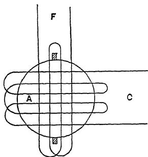
FIG. 156.—Circuits of single-phase commutator motor.
