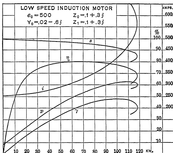
FIG. 20.—Low-speed induction motor, load curves.
