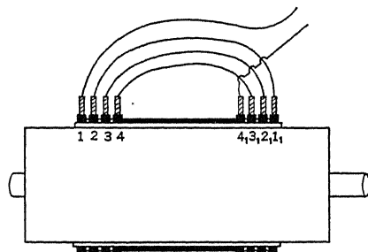
FIG. 225.—Multi-conductor unipolar machine, length section.
