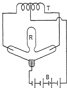
FIG. 101.—Mercury-arc rectifier, contact making.
