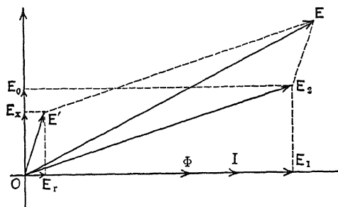
FIG. 175.—Single-phase commutator-motor vector diagram.
