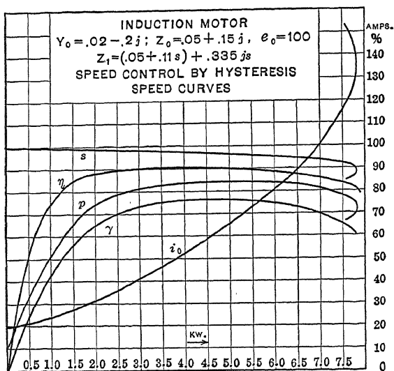
FIG. 3.—Load curves of induction motor with hysteresis starting device.
