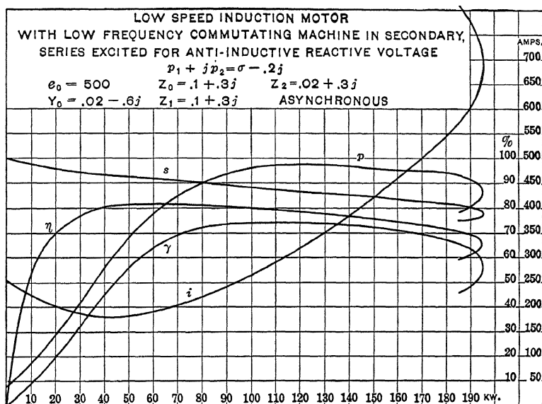
FIG. 31.—Load curves of high-excitation induction motor concatenated with commutating machine as reactive anti-inductive impedance.
