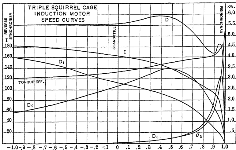
FIG. 16.—Speed curves of triple squirrel-cage induction motor.
