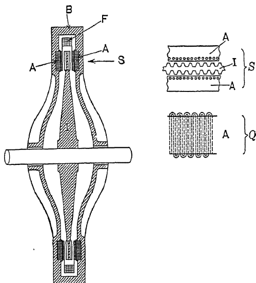
FIG. 138.—Alexanderson high frequency inductor alternator.
