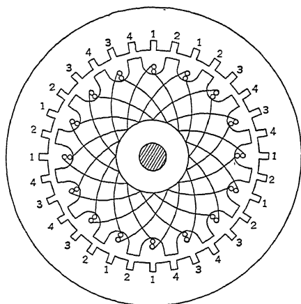
FIG. 142.—Induction type of high-frequency inductor alternator.
