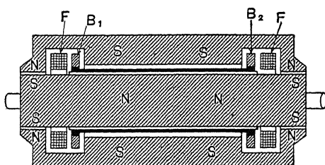
FIG. 223.—Double drum type of unipolar machine, section.
