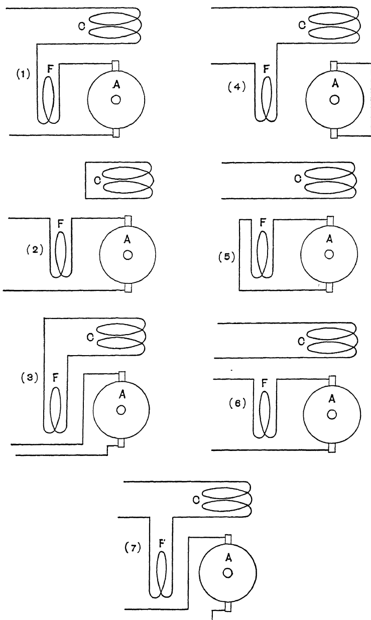
FIG. 164.—Types of alternating-current commutating motors.
