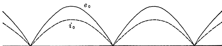
FIG. 74.—Rectified wave on non inductive load.
