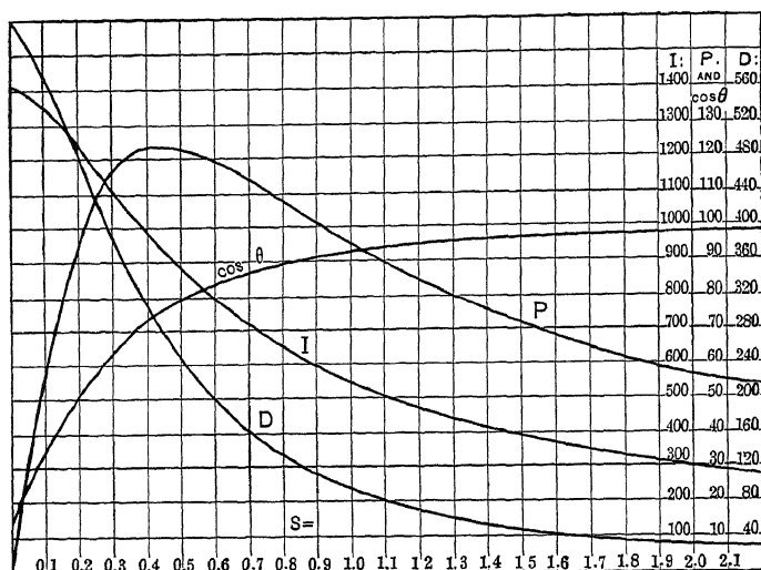
FIG. 173.—Single-phase commutator-motor speed characteristics.
