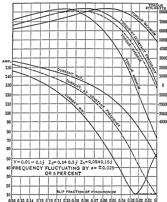
FIG. 50.—Effect of Frequency Pulsation on Induction Motor.
