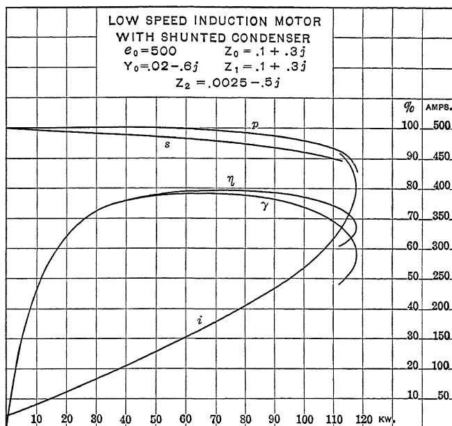
FIG. 32.—Load curves of high-excitation induction motor with shunted condenser.
