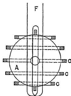
Fig. 163.—Eickemeyer inductively compensated series motor.
