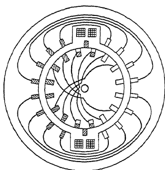
FIG. 160.—Fractional pitch armature winding.
