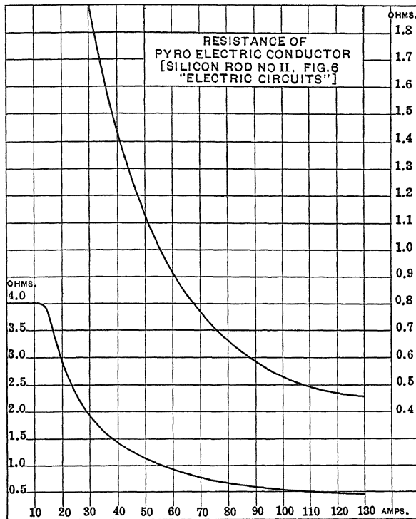
FIG. 6.—Variation of resistance of pyro-electric conductor, with current.
