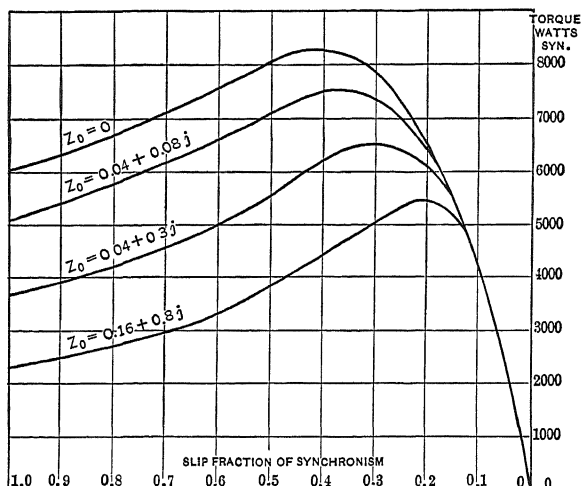
Fig. 47.—Induction-motor speed torque characteristics with a resistance of 0.15 ohm in secondary circuit.
