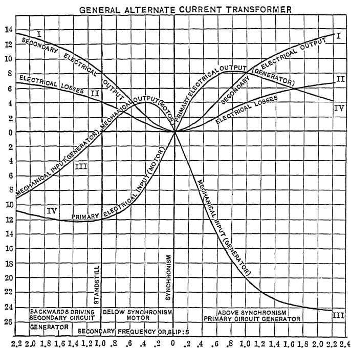
FIG. 62.—Speed-power curves of general alternating-current transformer.
