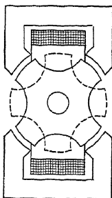
FIG. 127.—Four-polar reaction machine.
