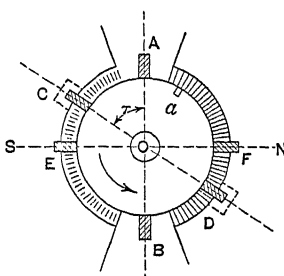
FIG. 196.—E.m.f. variation by shifting the brushes.
