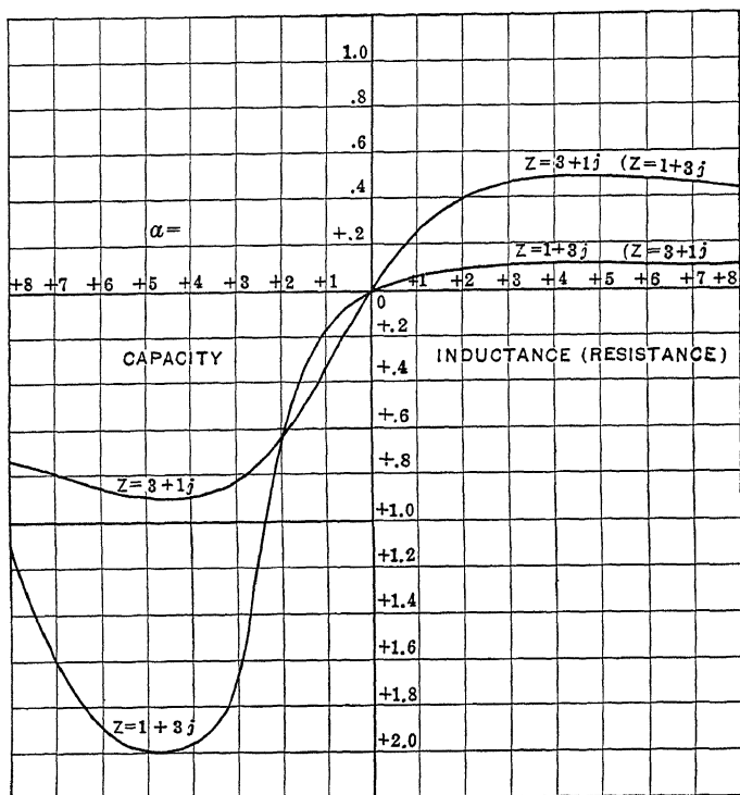
FIG. 37.—Apparent starting-torque efficiencies of phase-splitting device, parallel connection of motor circuits.
