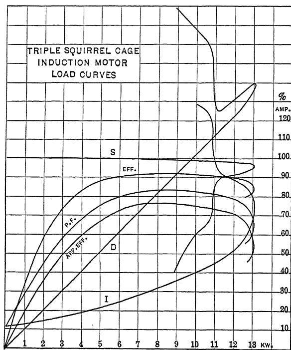
FIG. 17.—Load curves of triple squirrel-cage induction motor.
