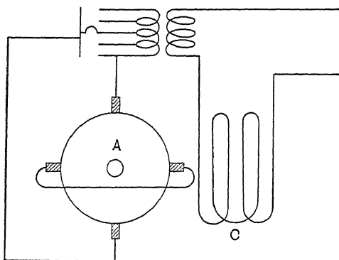
FIG. 184.—Winter-Eichberg motor.
