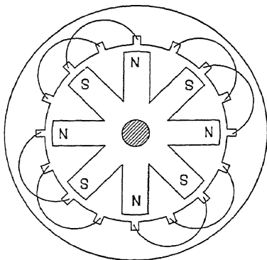
FIG. 135.—Revolving field alternator.
