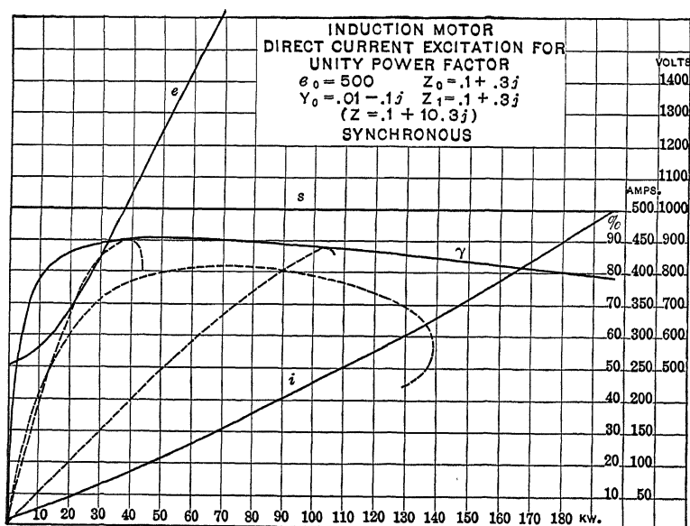
FIG. 23.—Load curves at unity power-factor excitation, of standard induction motor converted to synchronous motor.
