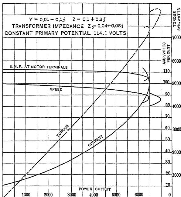
FIG. 43.—Induction-motor load curves corresponding to 110 volts at motor terminals at 5000 watts load.
