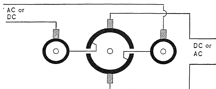
FIG. 73.—Rectifying commutator.
