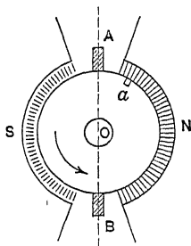
FIG. 195.—Diagram of commutating machine with brushes in the magnetic neutral.
