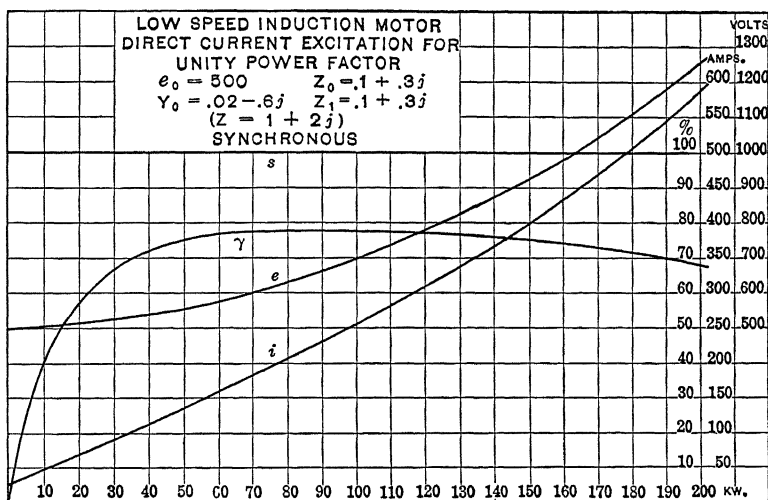
Fig. 26.—Load curves of low-speed high-excitation induction motor converted to synchronous motor, at unity power-factor excitation.
