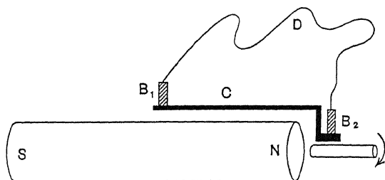
FIG. 216.—Diagrammatic illustration of unipolar machine with one high-speed collector.
