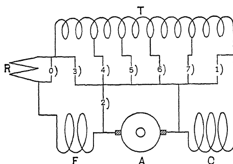
FIG. 181.—Alternating-current commutator motor arranged to operate either as series or repulsion motor.
