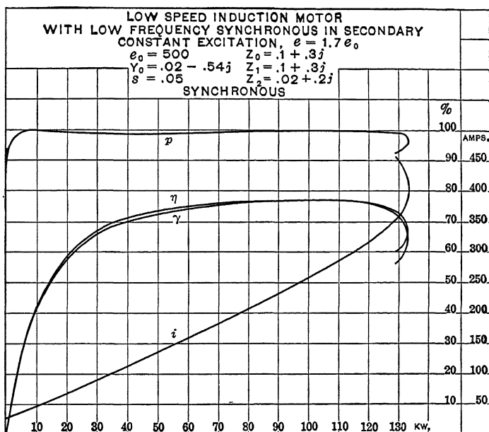
FIG. 30.—Load curves of high-excitation induction motor concatenated with synchronous, at constant excitation.
