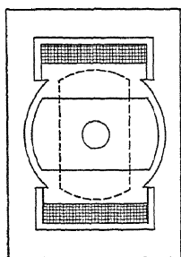
FIG. 126.—Bipolar reaction machine.
