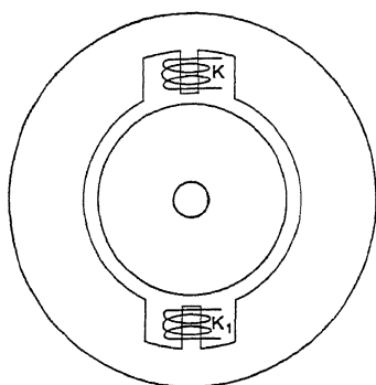
FIG. 172.—Commutation with commutating poles.
