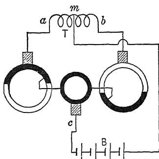
FIG. 97.—Contact-making rectifier with direct-current rotor.
