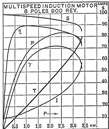
FIG. 11.—Load curves of multi-speed induction motor, low speed, eight poles.
