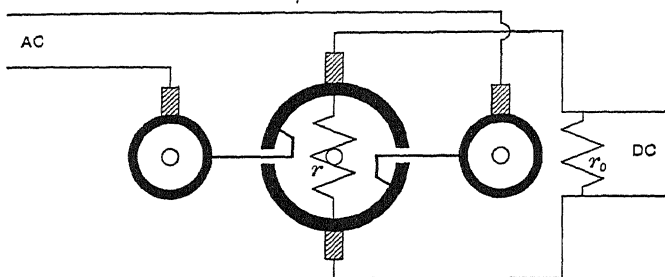
FIG. 78.—Rectifier with A.C. and D.C. shunt resistance for inductive load
