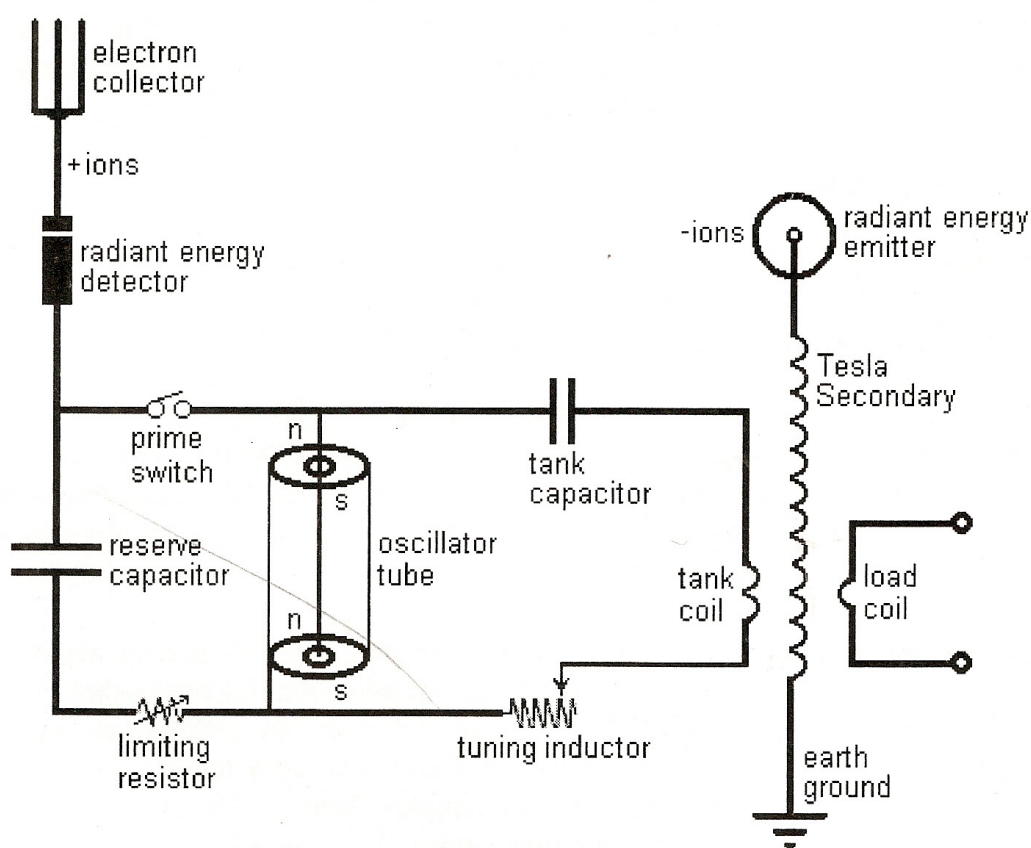
Proof of Concept - Figure 5
