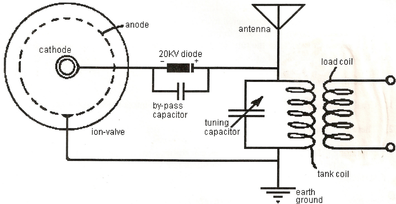
Basic Radiant Energy Receiver - Figure 3
