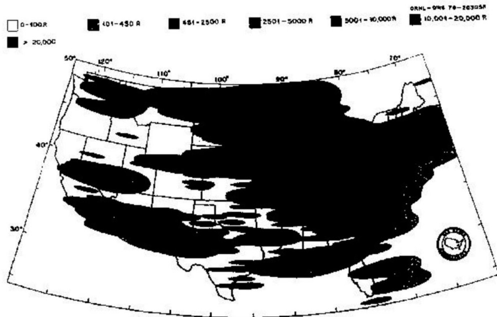
Fig. 4.1. Simplified fallout pattern showing total radiation doses that would be received by persons on the surface and in the open for the entire 14 days following the surface burning of 5050 megatons on the targets indicated, if the winds of all directions blew continuously from the west at 25 mph.
