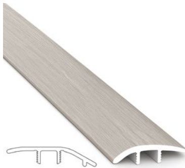
Reducer Oak Devonport 12"x48" | Fibrano w/ HydroWood
